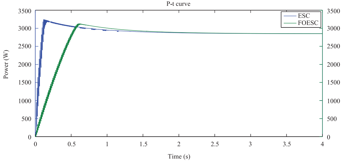
Fig. 13. Power-time curve comparison.
