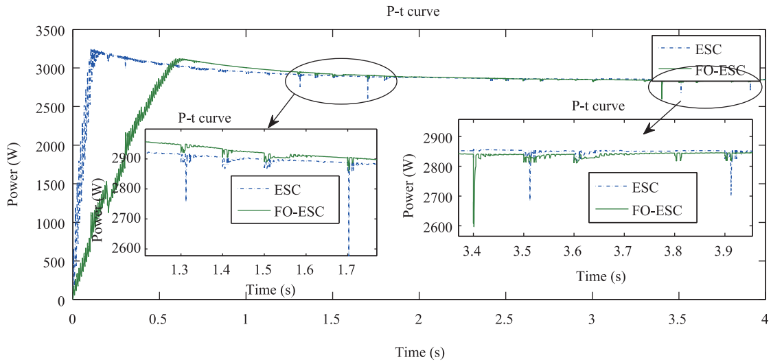
(a) Power-time curve comparison ESC
