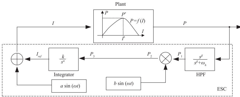
Fig. 6. Fractional order ESC (FO-ESC) without LPF.
