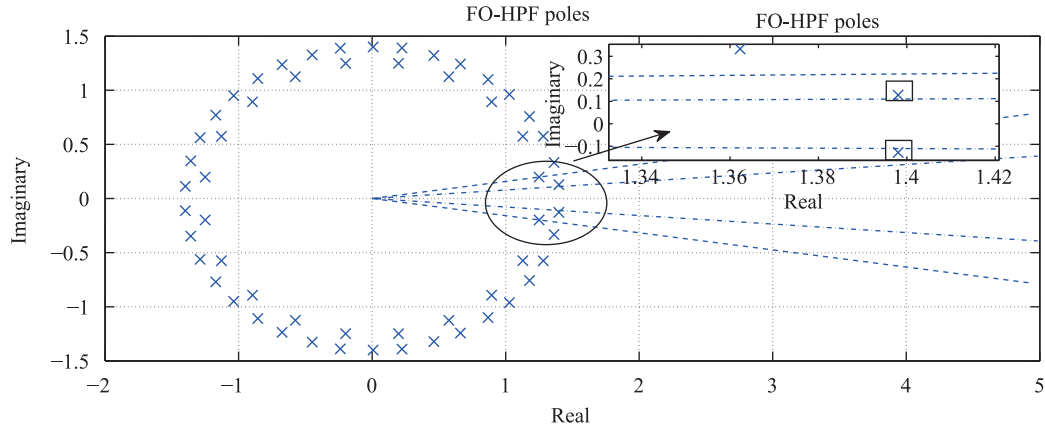
Fig. 11. Root map of FO-HPF-ESC.
