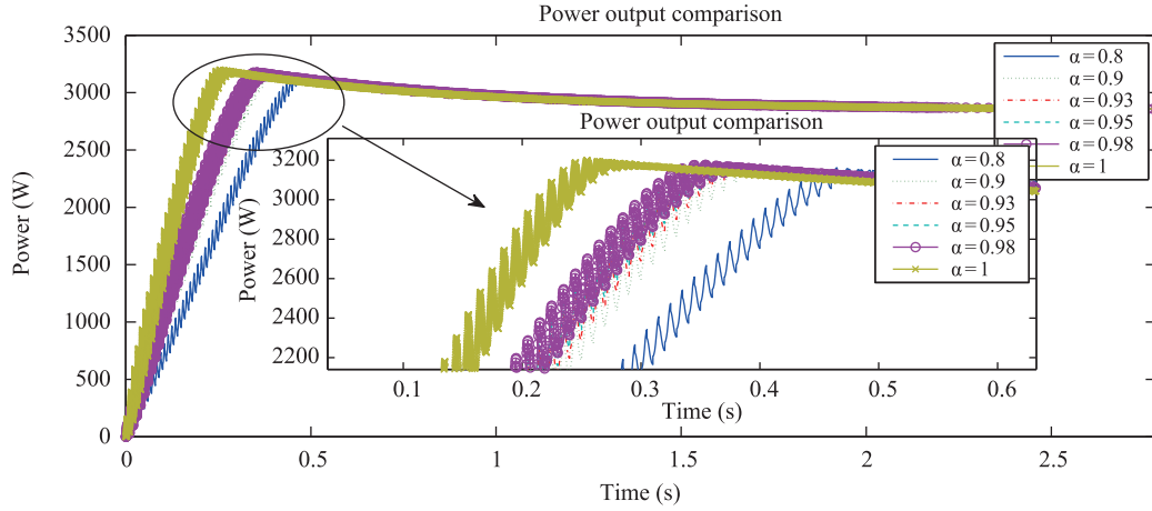
Fig. 12. Power output with FO-HPF-ESC.
