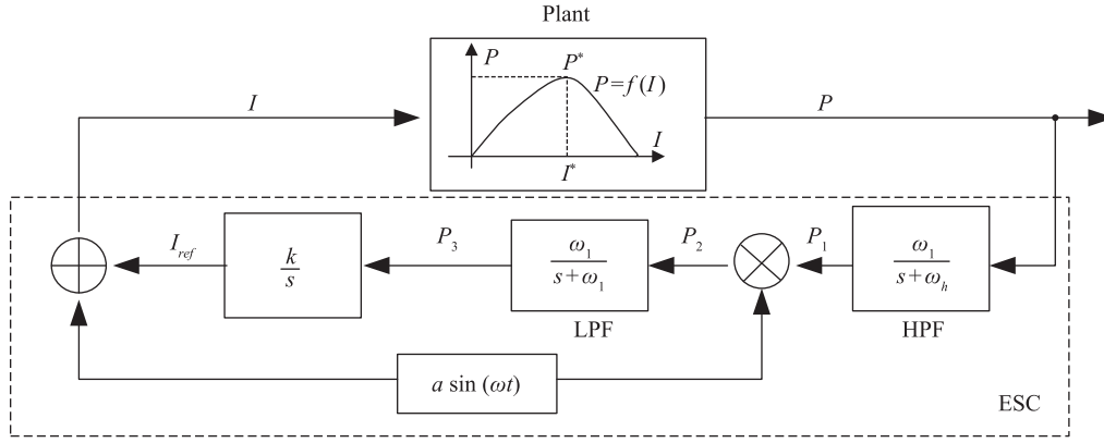
Fig. 4. General ESC control scheme.
