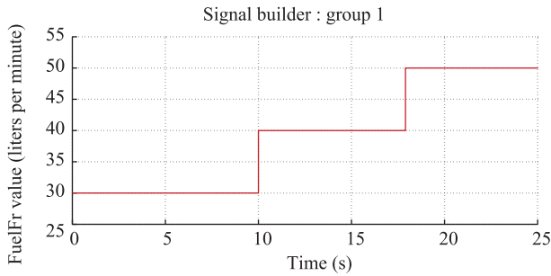
Fig. 17. Variant loads.
