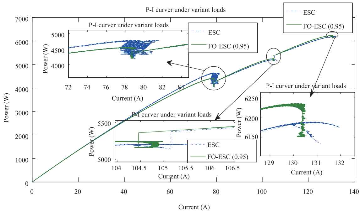
Fig. 16. MPPT performance under variant loads.
