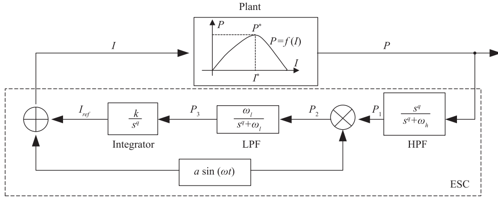
Fig. 5. Fractional order ESC (FO-ESC) control scheme.
