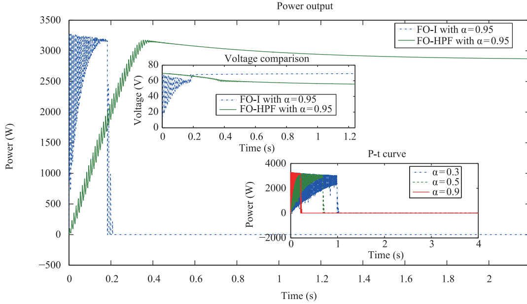
Fig. 10. Power/voltage output using ESC with fractional order integrator.
