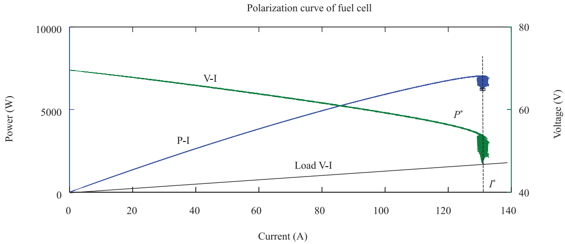
Fig. 2. Typical polarization curve and the maximum power point.
