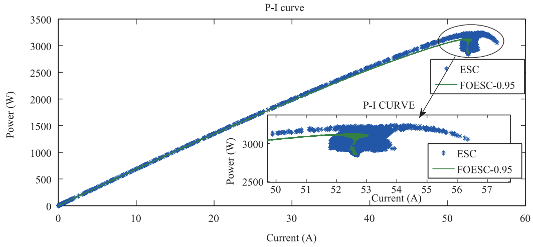
Fig. 14. Power output vs current during tracking.
