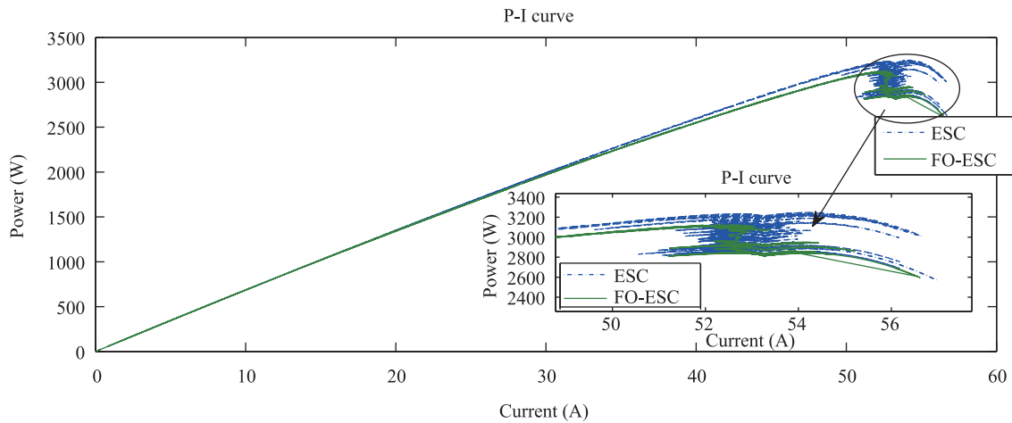
(b) Power-current curve comparison
