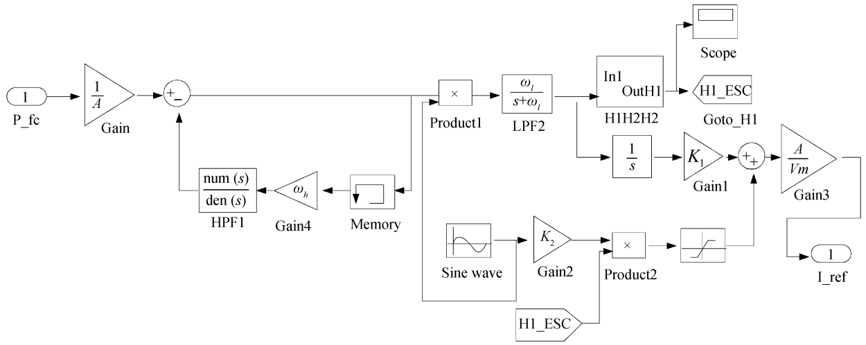
Fig. 7. MPPT controller with FO-HPF in Simulink.
