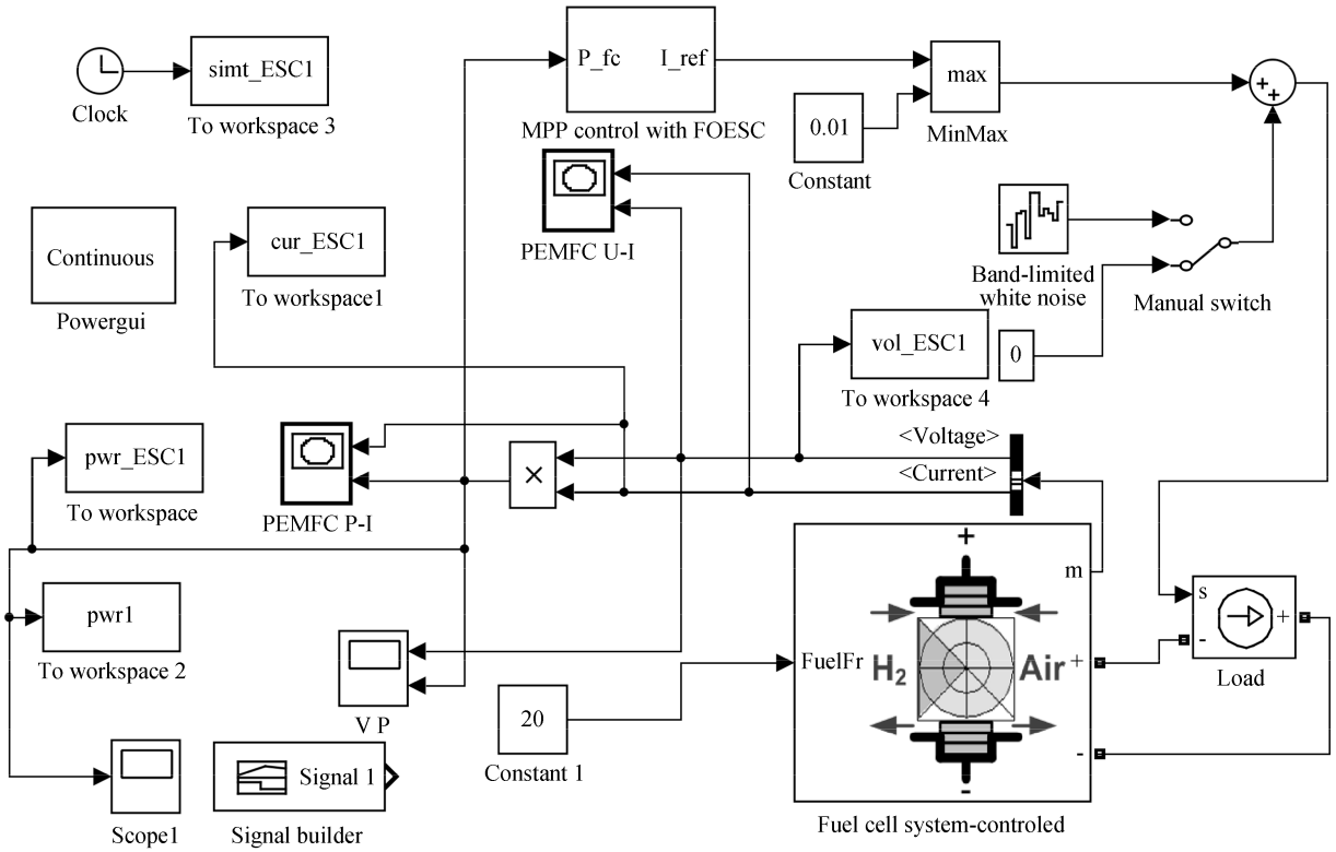
Fig. 8. Fuel cell with MPPT controller in Simulink.
