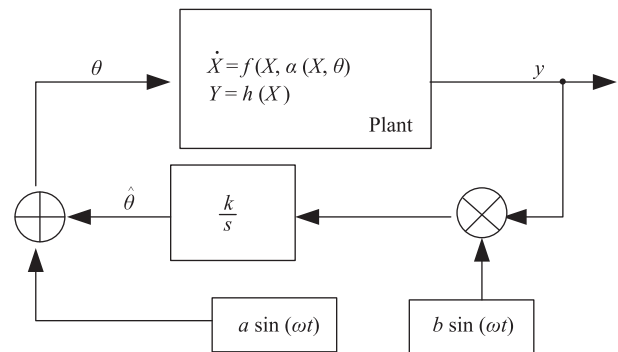
Fig. 3. The simplest peak searching scheme.
