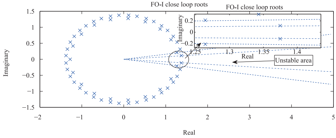
Fig. 9. Root map of ESC with fractional order integrator.
